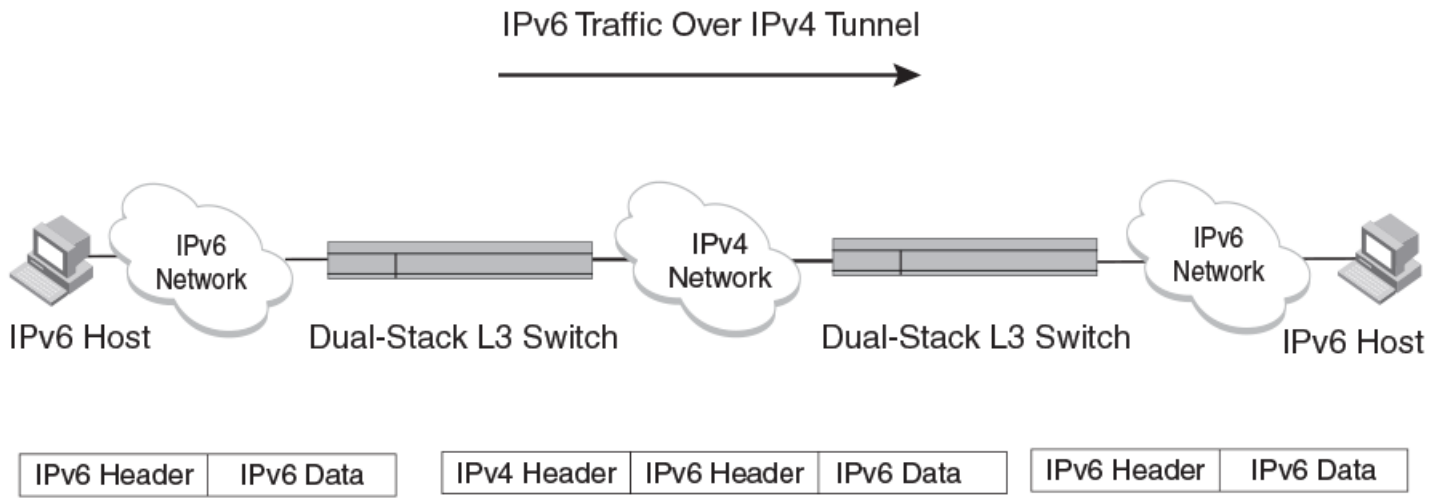
FIGURE 10 IPv6 Over an IPv4 Tunnel
